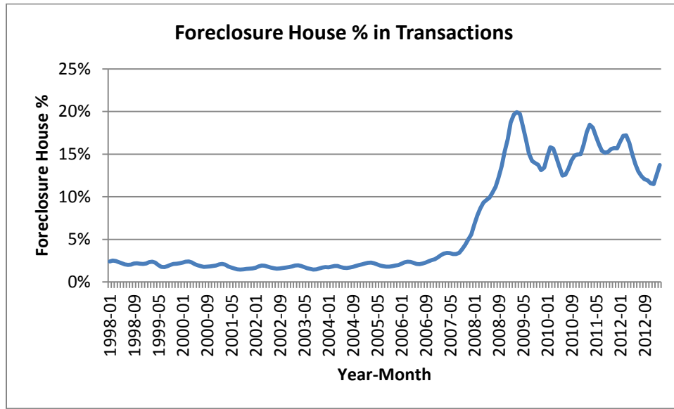
Figure 4: Monthly Foreclosure Homes as % of Transactions
